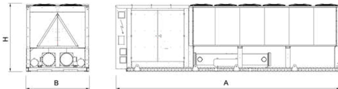
Dimensional drawing
